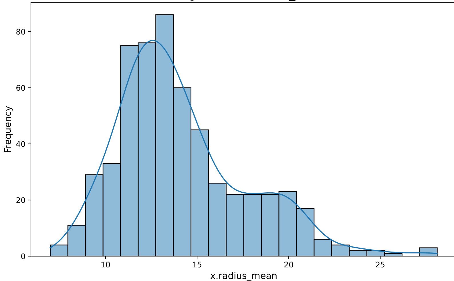
Histogram of x.radius_mean
